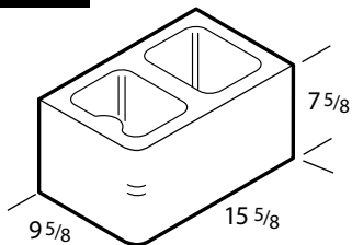
10 in. Single Bullnose*
