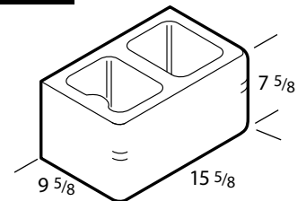
10 in. Double Bullnose* Face
