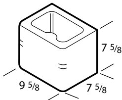
10 in. Two Qtr. / Half Block Double Bullnose*
